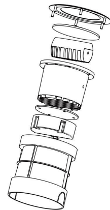
LED 埋地燈結構圖
